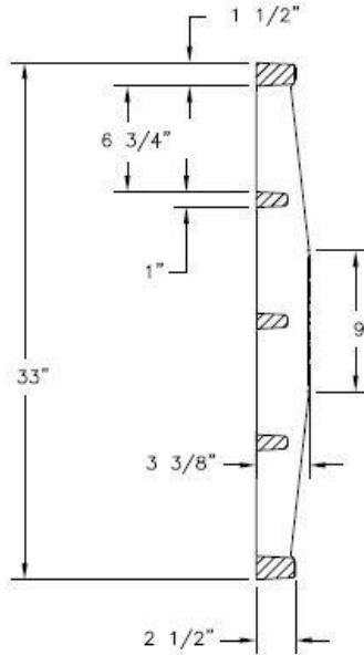
GRATE SECTION
