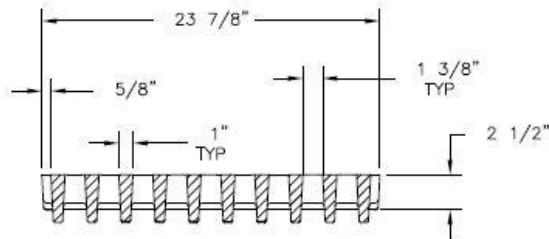
GRATE SECTION
